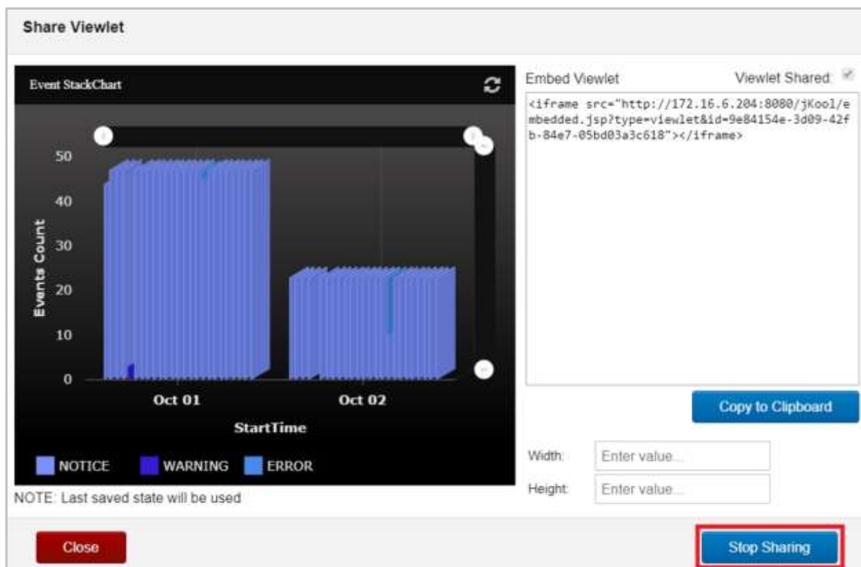
Figure 2.5.10-C. Stop Sharing a Viewlet
