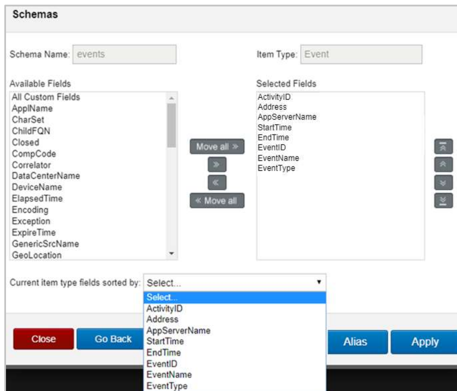
Figure 3.2.5-C. Add Fields for Schema
