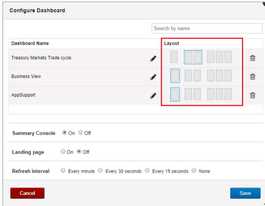
Figure 3.2.4.2-A. Configure Dashboard – Dashboard Layout
