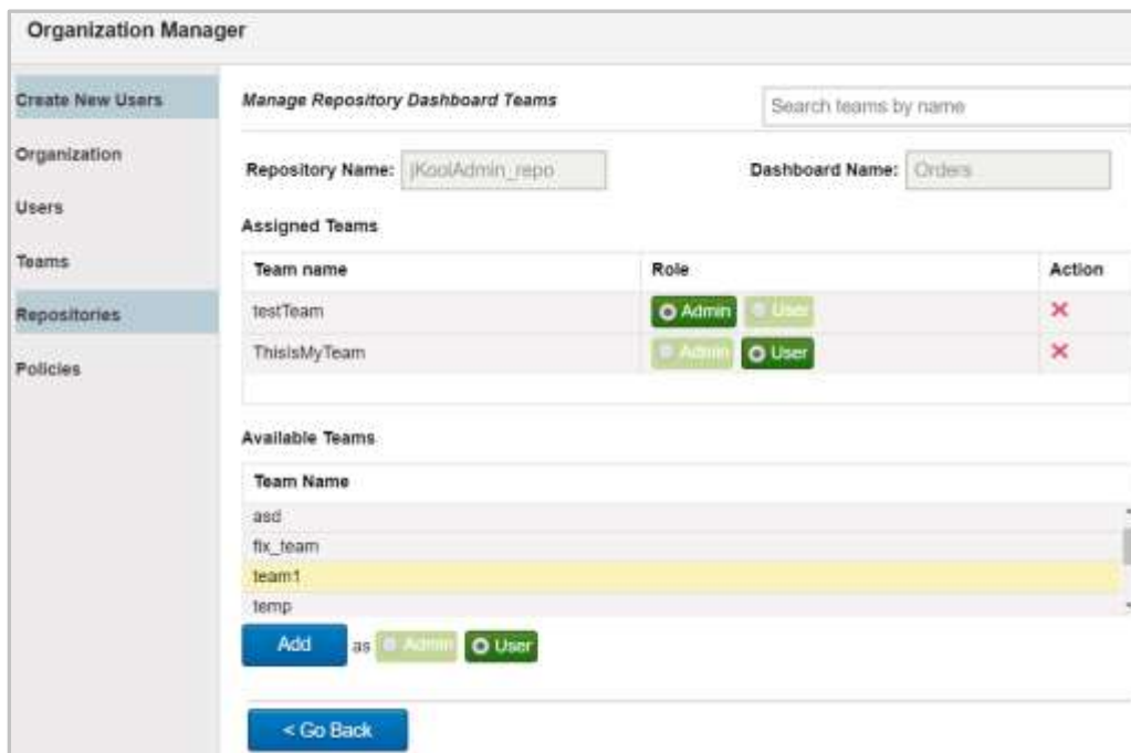
Figure 3.1.3.5.2-C. Manage Repository Dashboard Teams
