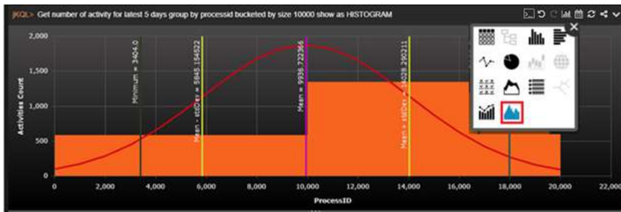
Figure 2.5.4.13-A. Histogram
