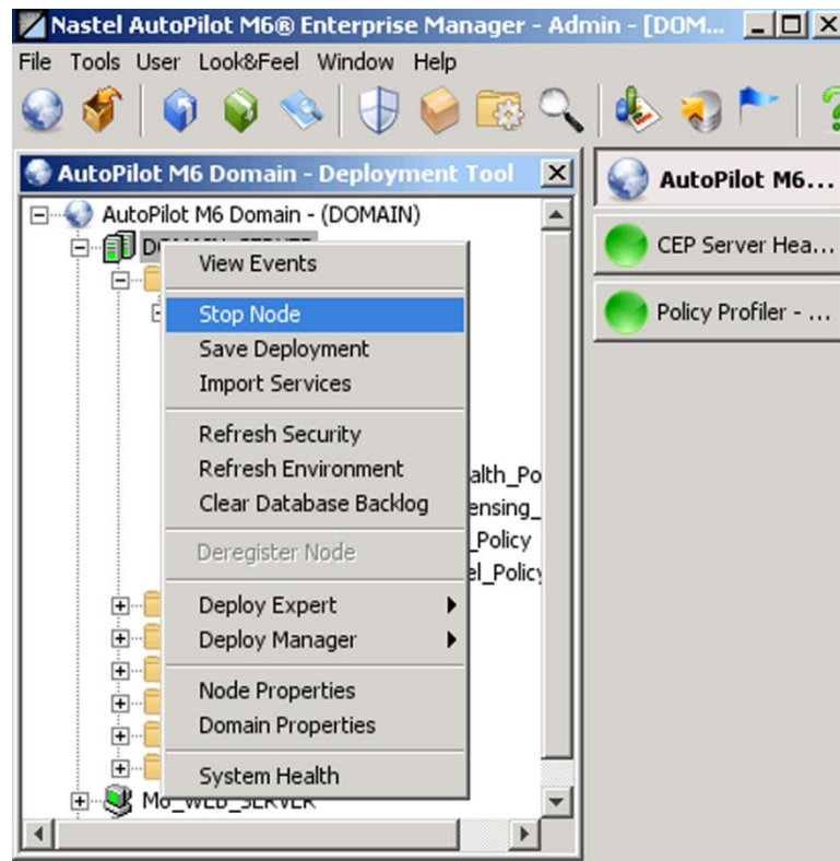
Figure 3-13. Stopping M6 on any Platform
