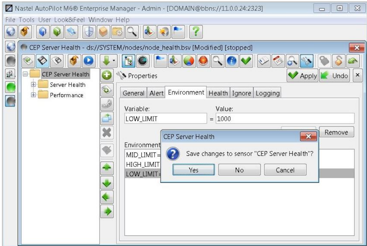
Figure 4-65-B. Adding a User Defined Environment Variable – Save Changes
