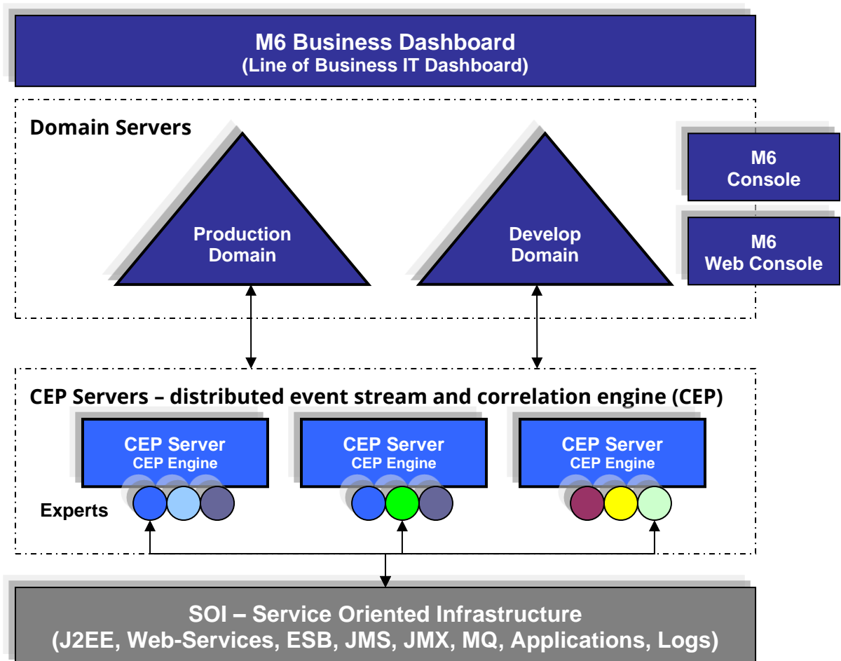
Figure 2-2. AutoPilot M6 Architecture
