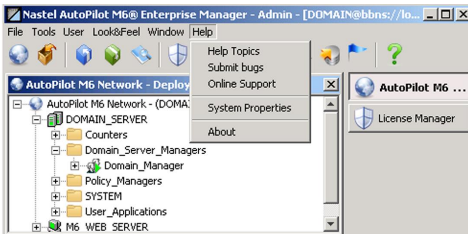
Figure 3-26. Help Menu
