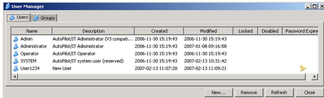
Figure 3-19. User Manager
