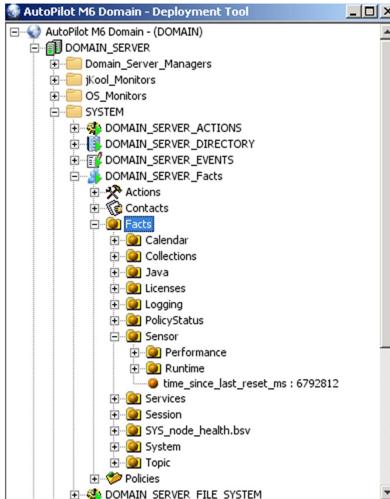
Figure 2-10. Facts View
