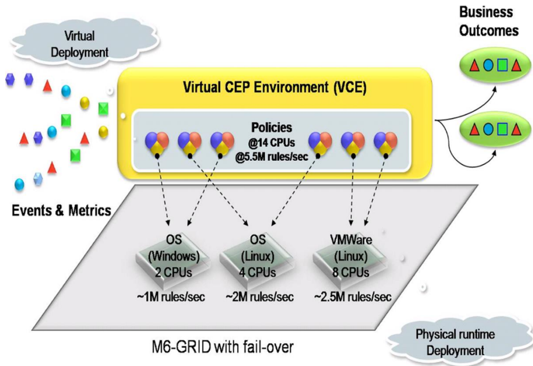
Figure 2-1. Virtual CEP
