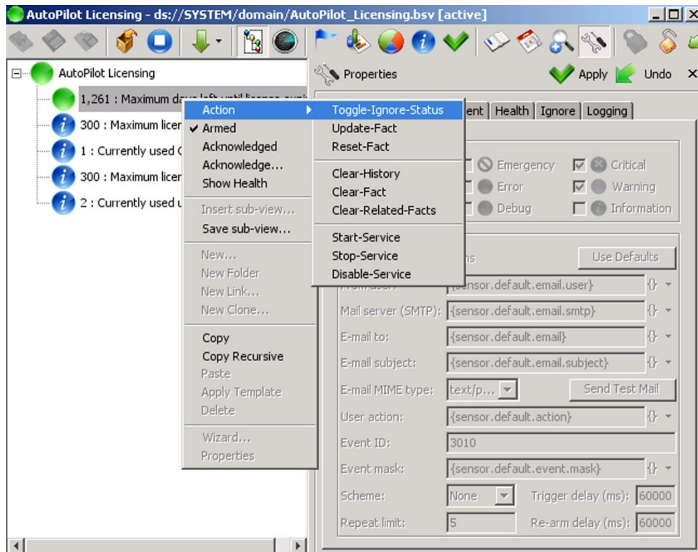
Figure 4-99. Toggle-Ignore-Status Menu
