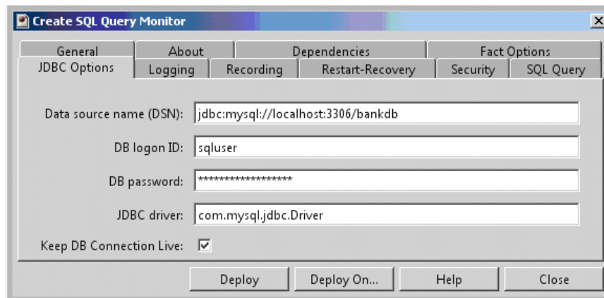
Figure 4-33. SQL Query, JDBC Options Tab
