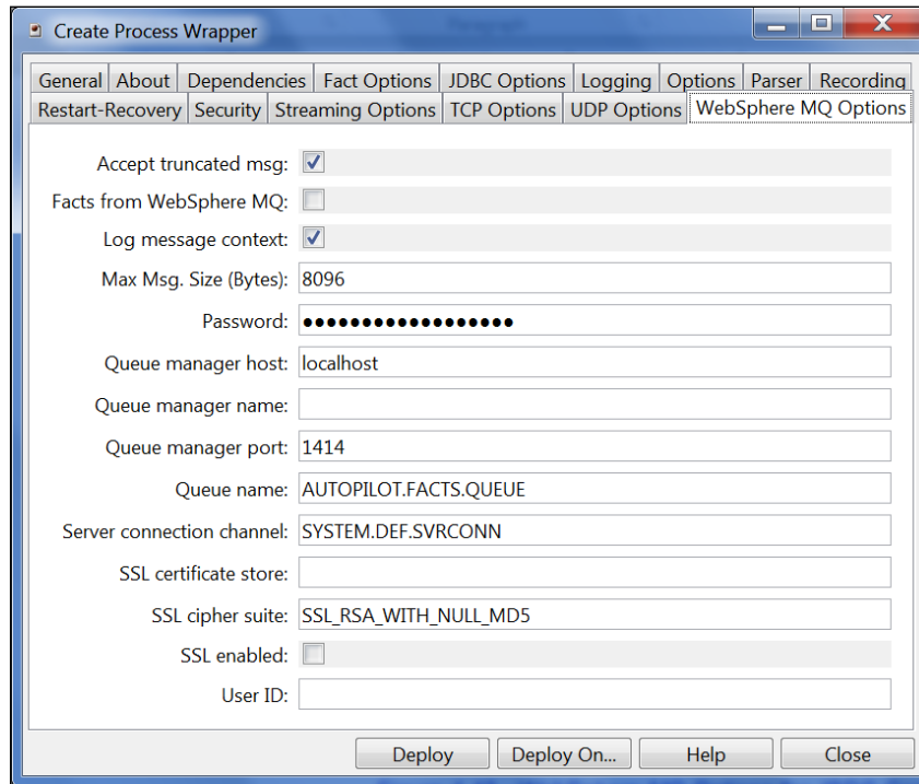
Figure 4-43. WebSphere MQ Options for JDBC Configuration
