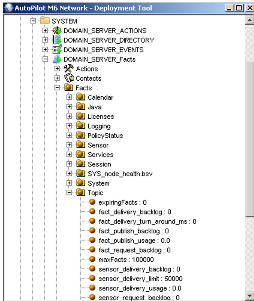
Figure 5-2. CEP Server, Domain Server Facts
