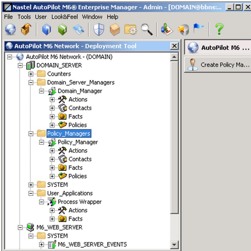
Figure 2-8. Policy View
