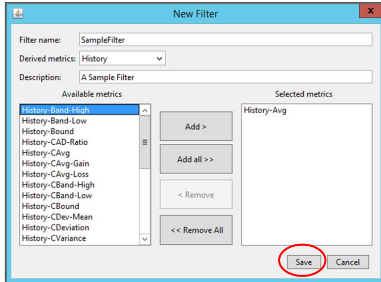
Figure 4-138. New Filter
