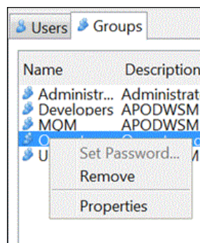
Figure 4-10. Groups Sub-menu
