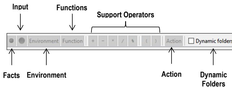
Figure 4-81. Supported Operators
