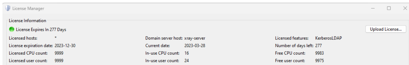
Figure 4-1. License Manager
