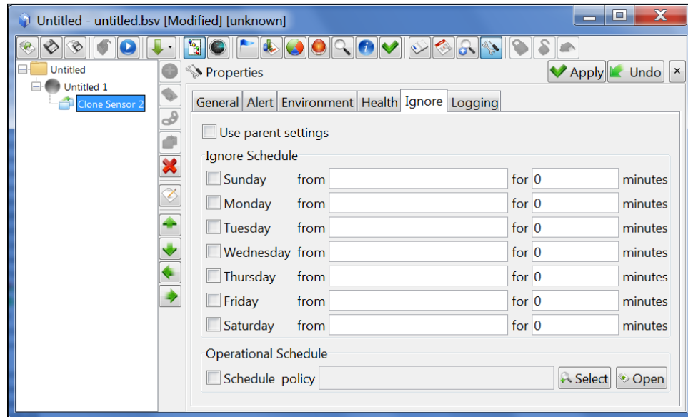
Figure 4-88A. Clone Sensor Properties
