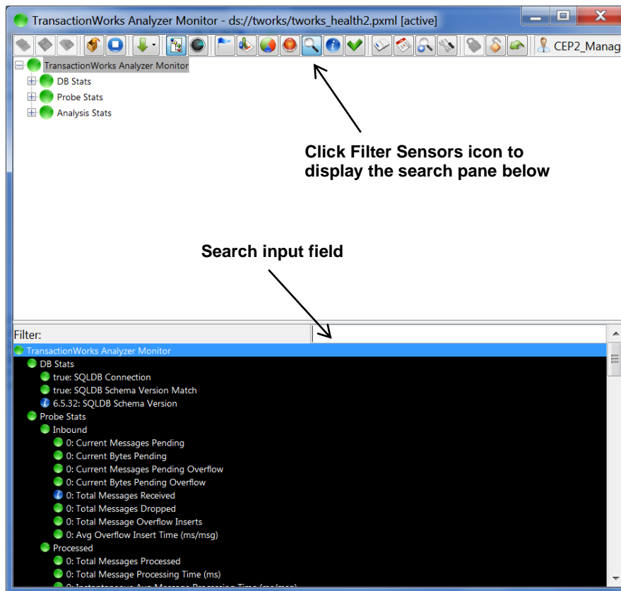
Figure 4-61B. Sensor Search List
