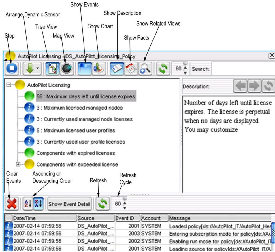
Figure 3-33. Getting Around M6 Web Console
