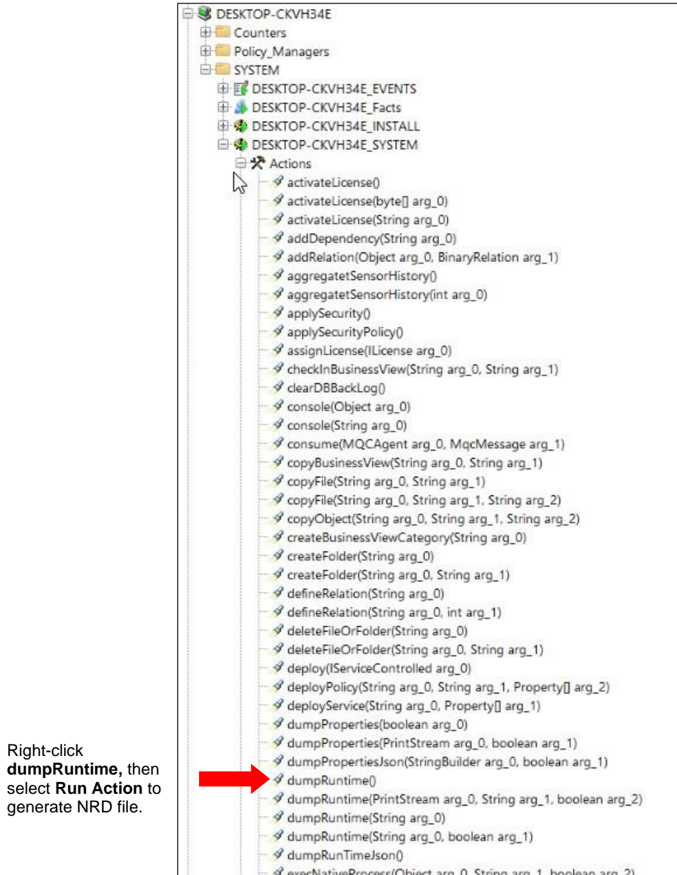
Figure 6-7. Generate NRD File
