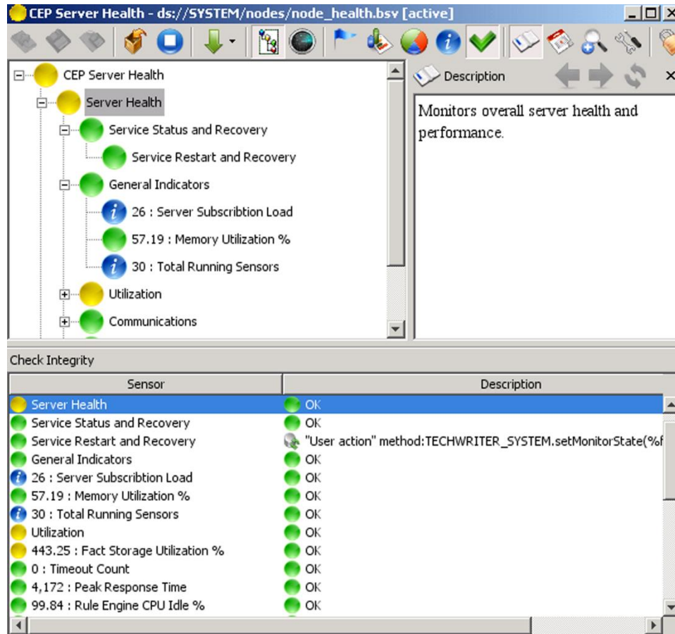
Figure 4-112. Business View Sensor Integrity
