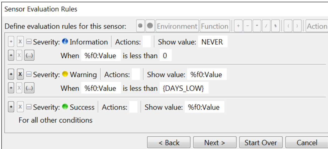
Figure 4-74. Sensor Rules
