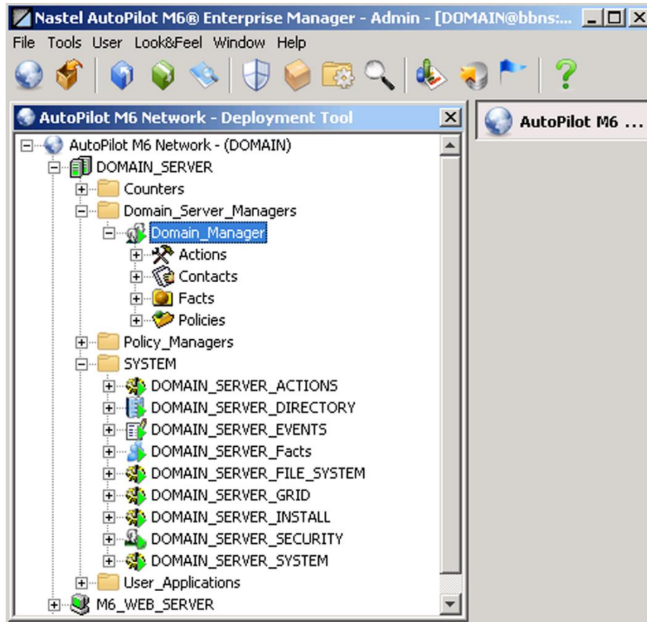
Figure 3-9. User Console
