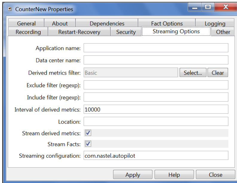
Figure 4-136. Streaming Options
