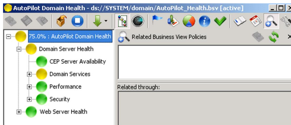
Figure 4-116. Related Views
