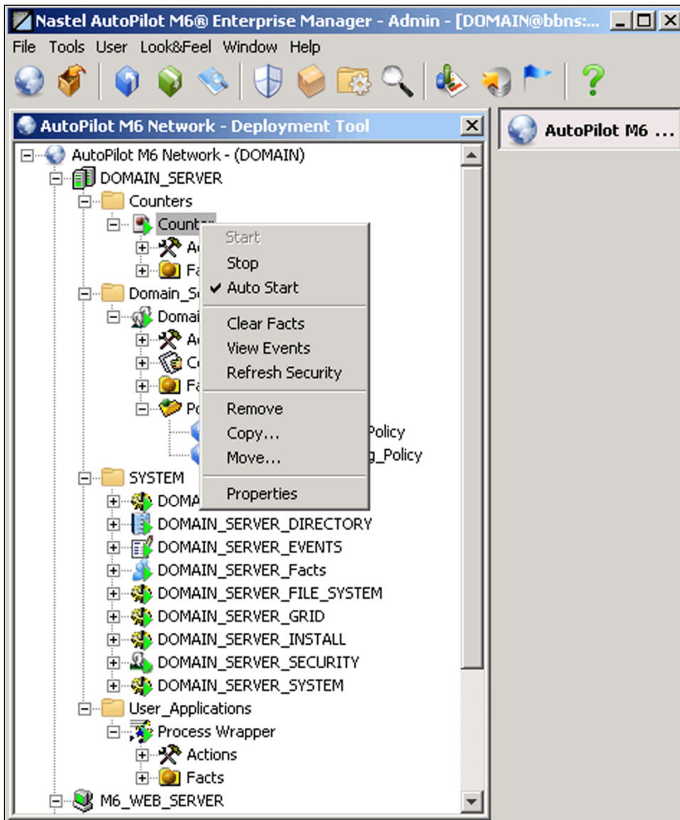
Figure 2-6. Management Services View
