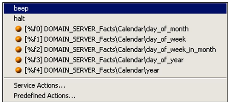
Figure 4-76. Actions
