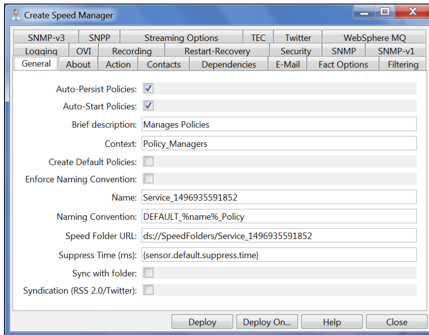
Figure 4-54. Deploying Managers
