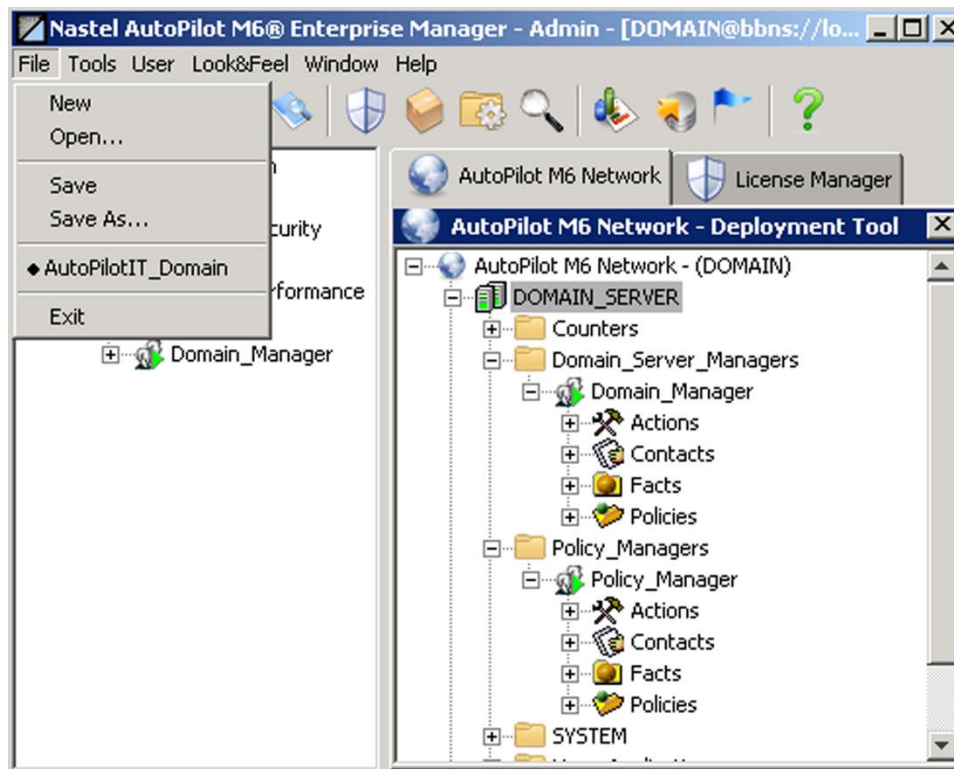
Figure 3-15. M6 User Console - File Menu
