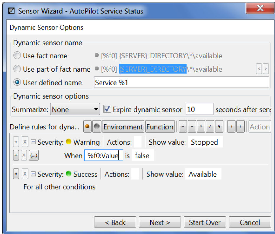
Figure 4-83. Dynamic Sensor Options
