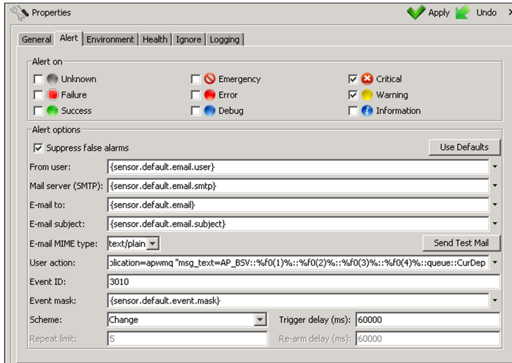
Figure 4-135. Example of Queue Depth Manual Acknowledgement Alert Screen
