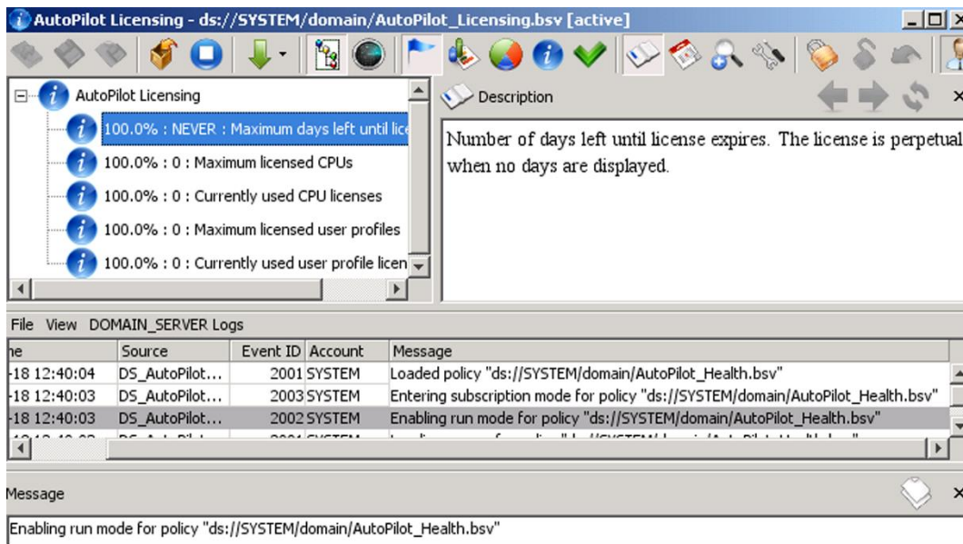
Figure 4-121. Sample View of an Event Log
