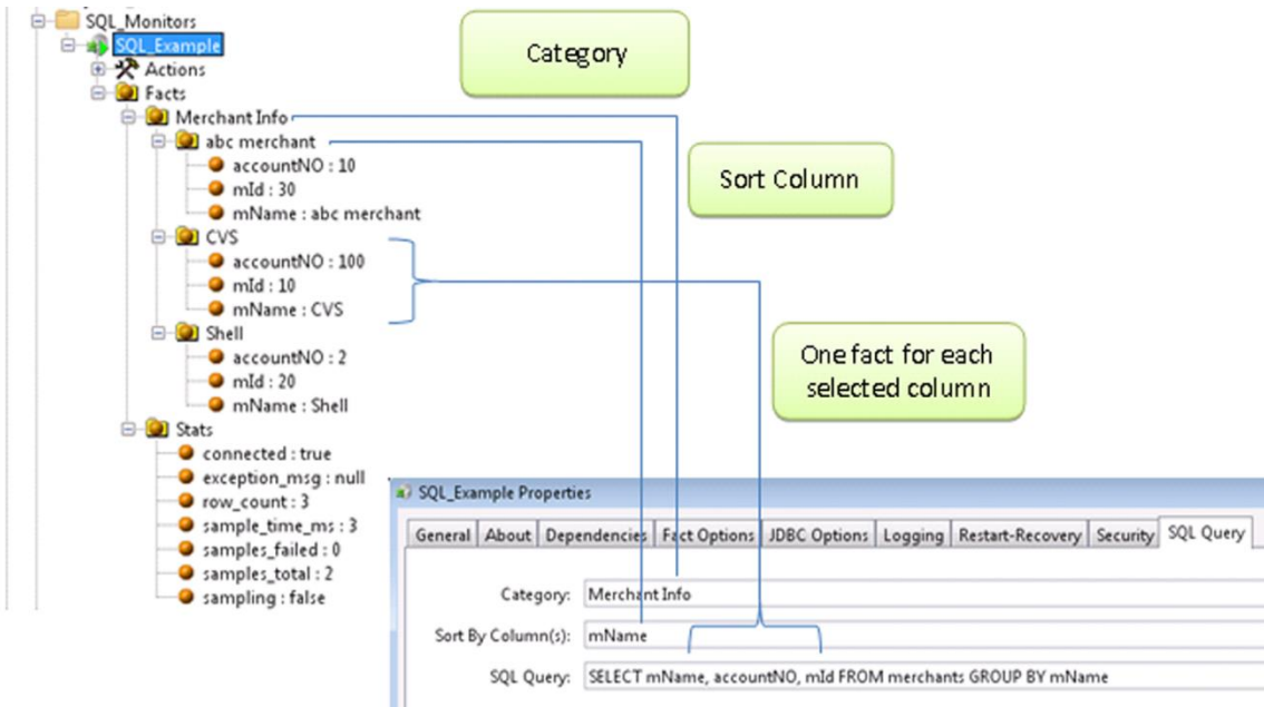
Figure 4-35. SQL Query Facts
