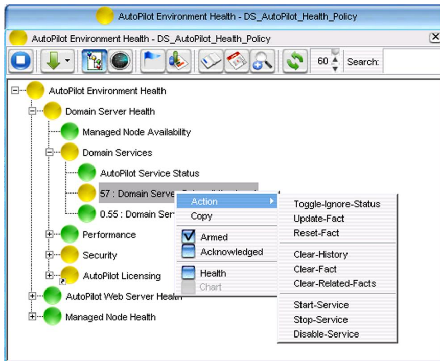
Figure 3-35. M6 Web Console Operator Actions
