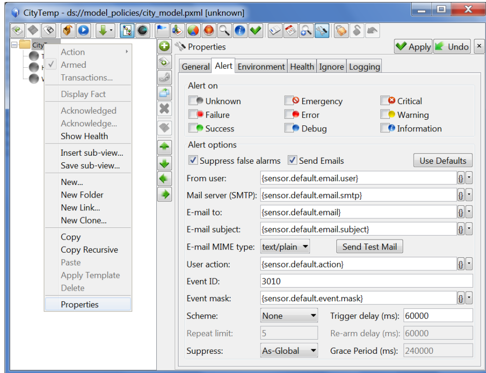
Figure 4-70. Changing Sensor Properties
