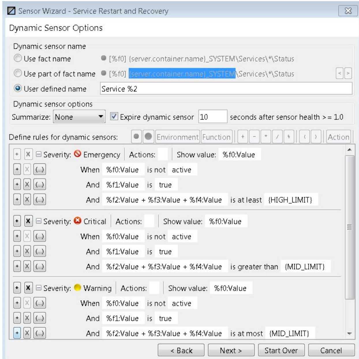
Figure 4-65-C. Policy CEP Server Health Sensor Wizard Service Restart and Recovery
