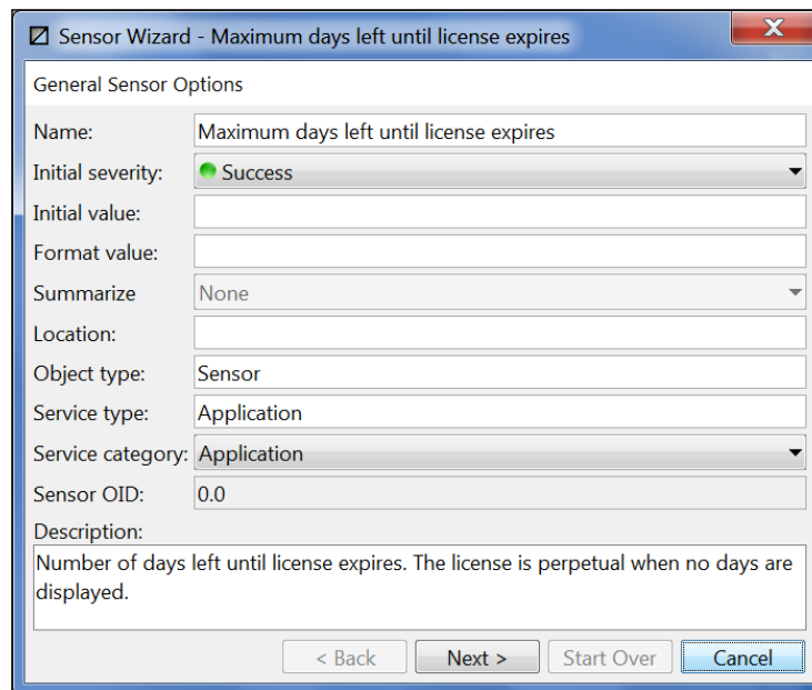
Figure 4-72. Create a New Sensor - General Screen
